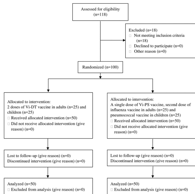
Fig 1. Consort diagram.
